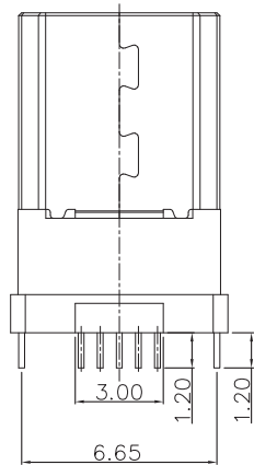
DETAILED A SCALE 1:1
