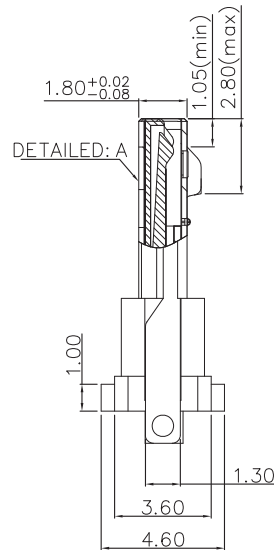
DETAILED A SCALE 1:1
