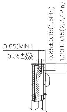
DETAILED A SCALE 1:1
